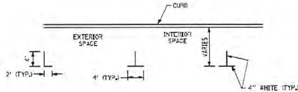
Parallel On-Street Parking Detail Source – NYSDOT
