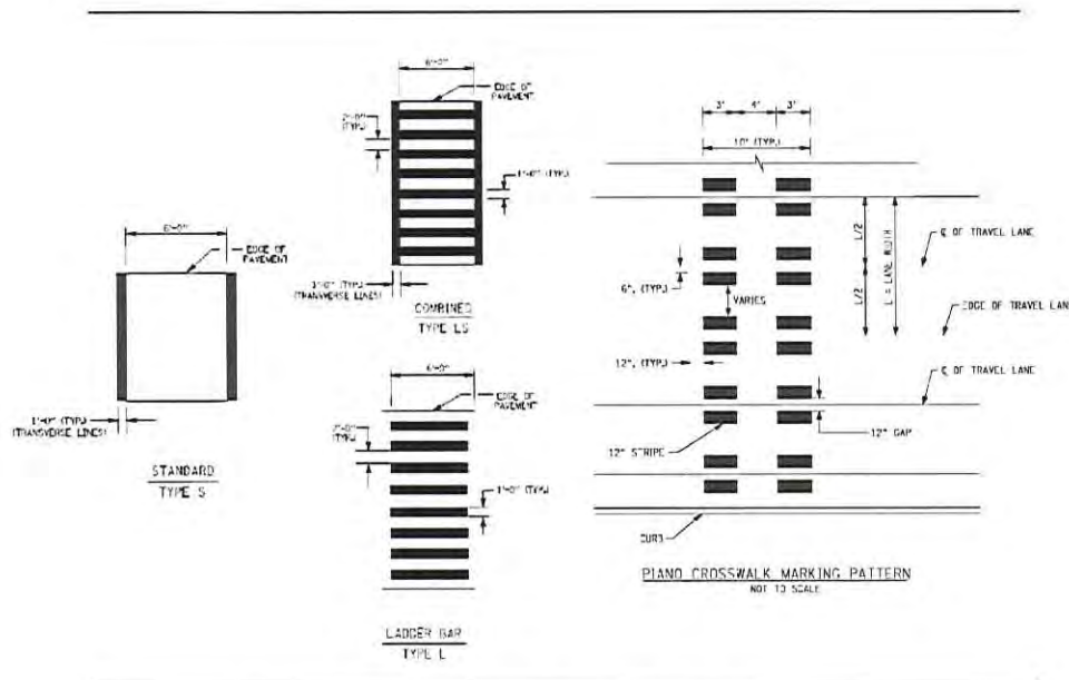
Typical Crosswalk Marking Details
