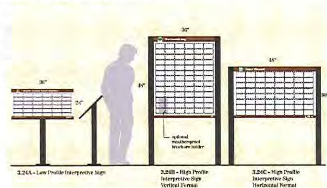
Interpretive Signing Formats - Source, NYS Scenic Byways Sign Manual
