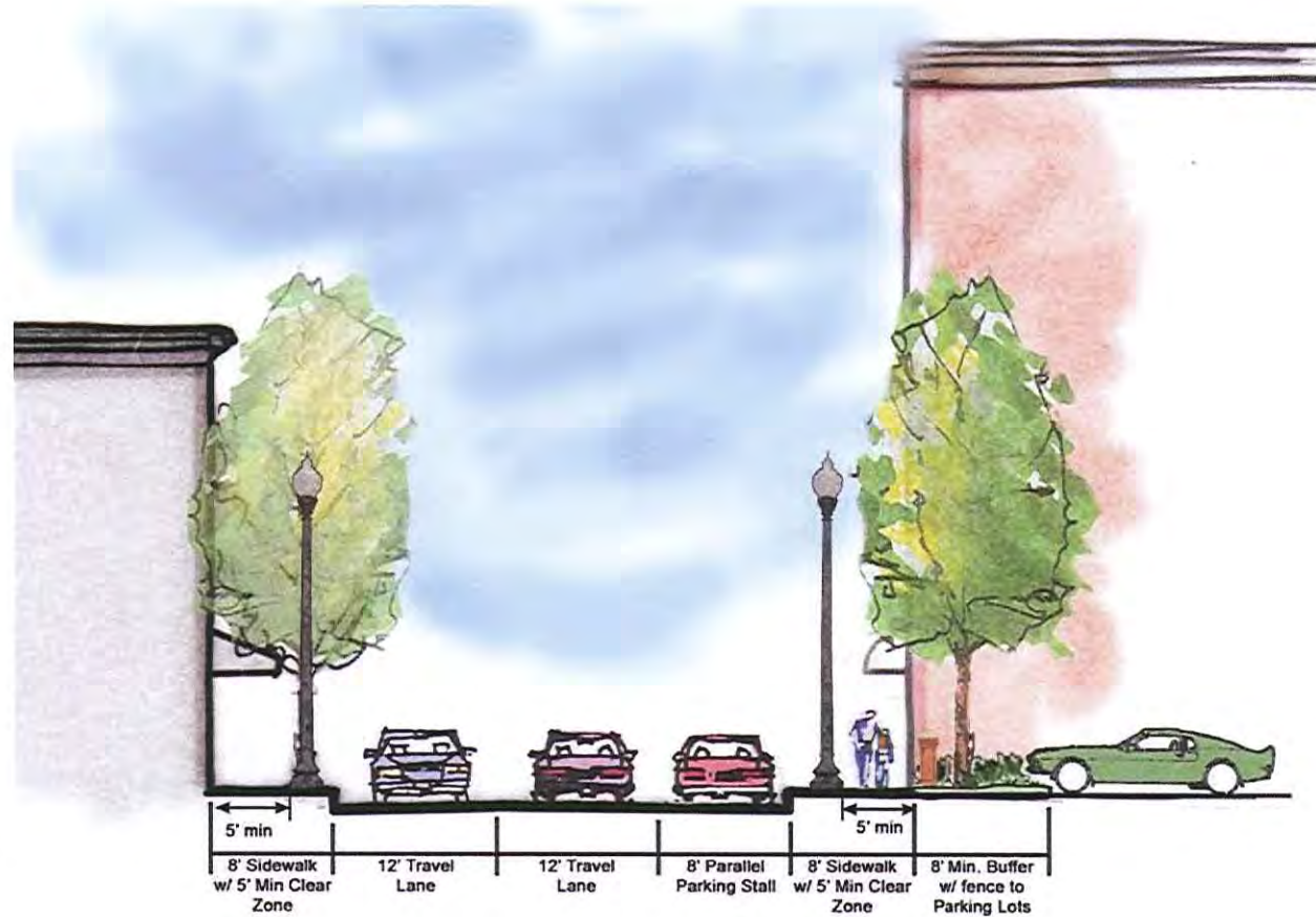
Section Detail Second Street, City of Jamestown
